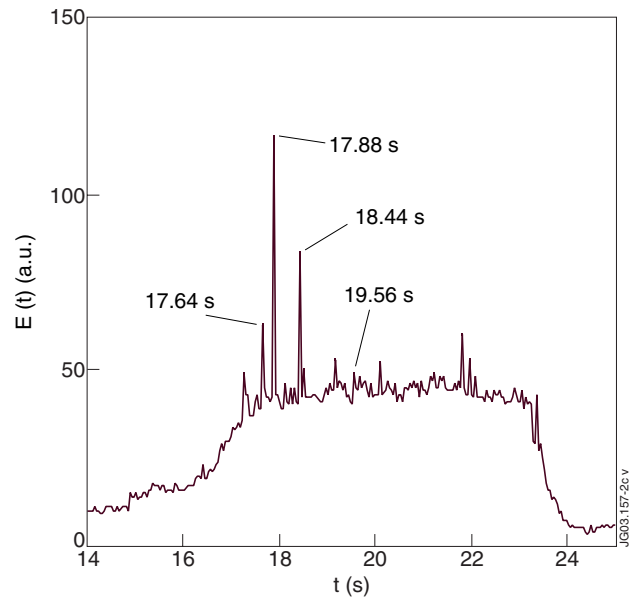
Figure 2 : Time trace of the emission of visible light. The emission saturates at a value of 256. Spikes are associated to ELMs. The rise of the background emission corresponds to the H-mode phase of the discharge. The various times highlighted on the plot correspond to the time used in fig. 3 and fig. 4 to draw the emission profiles.
