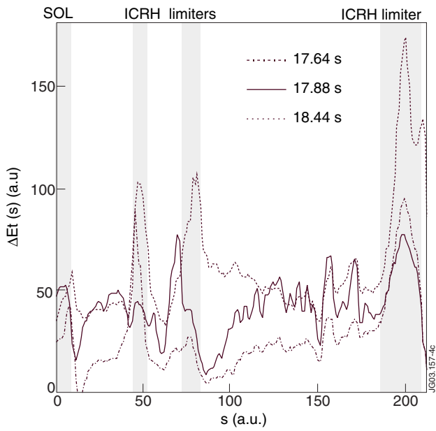
Figure 4 : Emission profile from a line following a rotational transform on the low field side of the vessel. Strong emission regions are highlighted by the shaded areas, high-field SOL, and three ICRH guard limiters. The three selected times correspond to emission peaks, see fig. 2.
