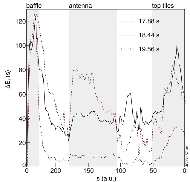
Figure 3 : Emission profile from a poloidal line running from the divertor to the top protection tiles at the intersection of a poloidal plane and the outer wall. Strong emission regions are highlighted by the shaded areas, baffle, ICRH antenna and top tiles. The three selected times correspond to emission peaks, see fig. 2.
