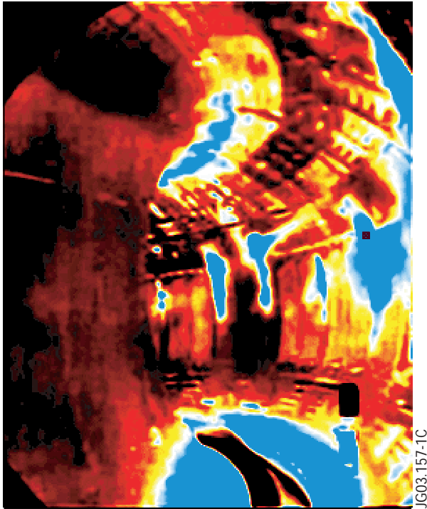
Figure 1 : Image of the visible light emission in JET after filtering. This image is the difference between the average of the emission during the ELMs and the average of the emission when no ELM is detected. The intensity is in arbitrary units and the colour ordering is the following, black, red, yellow, white, blue, black being “cold” and blue “hot”. The “cold” regions are those where the visible emission has decreased or weakly changed. The “hot” regions correspond to significant emission increase during the ELMs. In this treatment contrast is enhanced. Lettering on the figure locates the various components, A the top protection tiles, B one of the ICRH guard limiters, C outboard baffle and low field-side SOL, D inboard baffle, E inner wall, F ICRH antenna. The point identified by small crossed square is that used in fig. 2 to plot the time trace of the emission.
