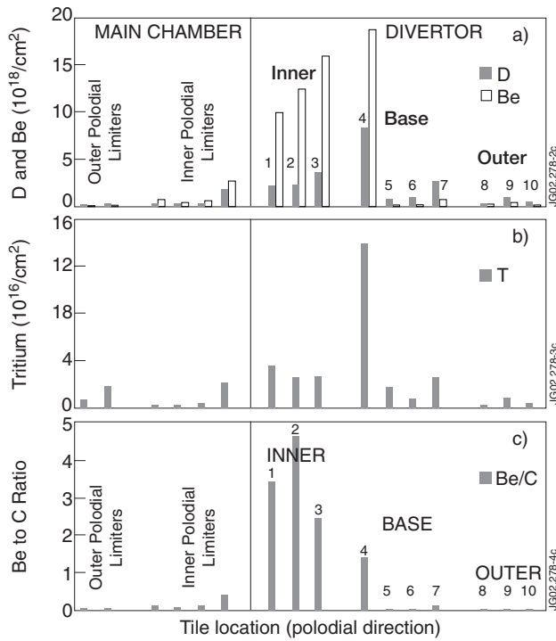
Figure 3: Concentration and relative distribution of species on plasma facing surfaces in the main chamber and the divertor: (a) deuterium and beryllium, (b) tritium, (c) beryllium-to-carbon ratio.
