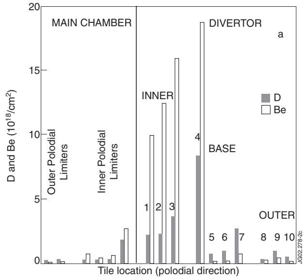
Figure 4: Distribution and concentration of deuterium and beryllium on tiles 3 and 4 of the divertor.
