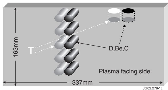
Figure 2: Sampling procedure for the determination of tritium with a full combustion method and other elements (D, Be, C) by surface analysis.
