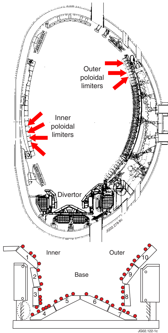
Figure 1: Schematic cross-section and location of tiles and samples in the JET (a) vessel and the (b) Mk-IIA divertor.
