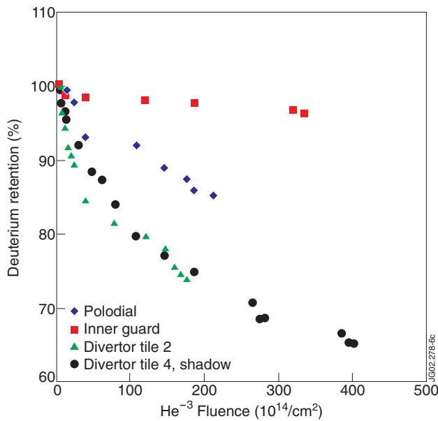
Figure 5: Detrapping of deuterium
