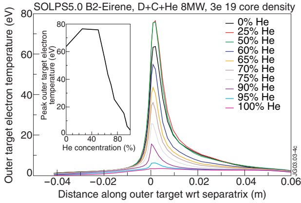
Figure 4. Electron temperature at the outer target for a number of code runs with varying helium concentration. Inset is the peak outer target electron temperature as a function of the helium concentration. 8MW simulations of the JET DOC-U configuration.
