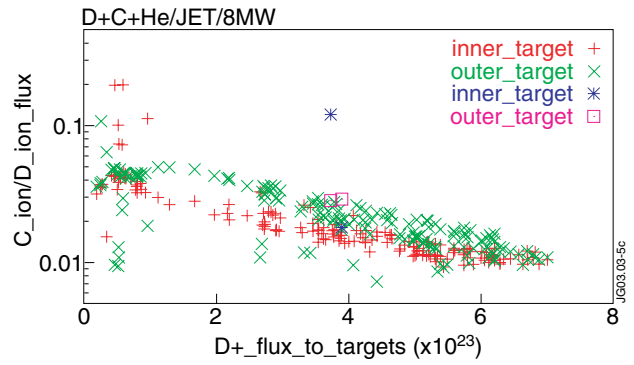
Figure 5. Ratio of C ion fluxes to the D ion flux for the inner and outer targets versus the sum of the D ion flux to both targets. The two pairs of selected points correspond to a case where the chemical sputtering coefficient was artificially increased from 1% (the two points in the band) to 10% (which has the point for the inner target raised well above the band of points). There are also some interesting points with large in/out asymmetries between the C-to-D flux ratios at low D+ flux values: these plasma are dominated by strong volume recombination, particularly in the inner divertor.
