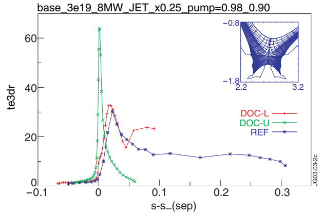
Figure 2. Outer target electron temperature profiles from a SOLPS5.0 B2-Eirene simulation. Inset is a zoom of the divertor region of the reference grid. (The DOC-L and DOC-U grids are shown as insets figure 1.)
