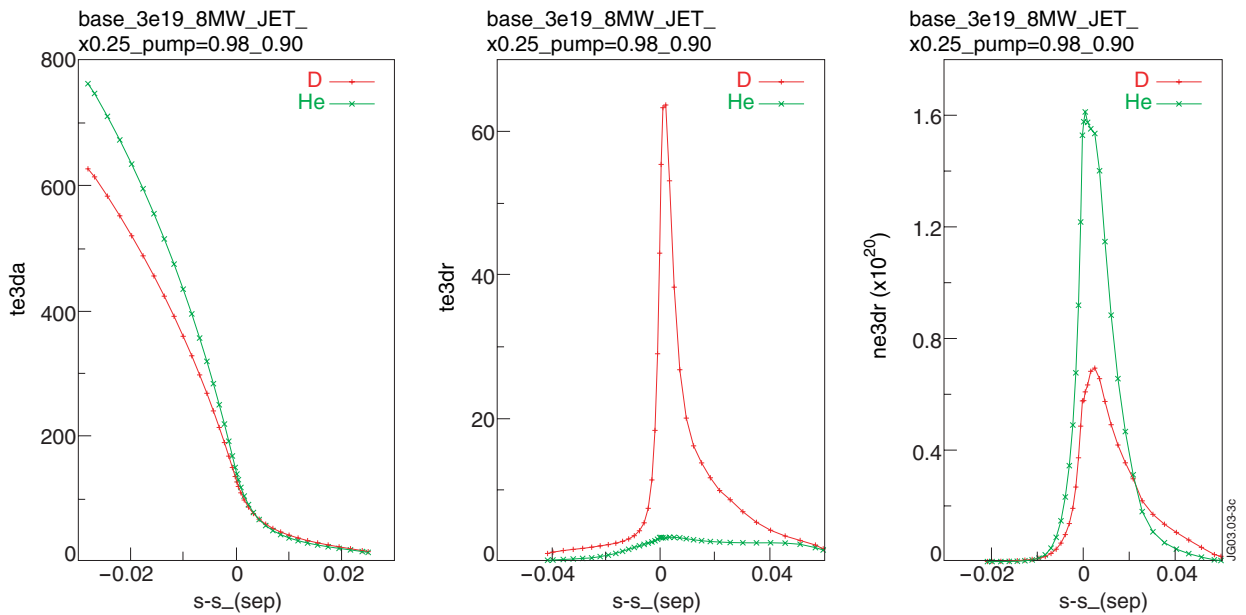
Figure 3. D and Helium give very different target profiles. 8MW simulations of the JET DOC-U configuration.
