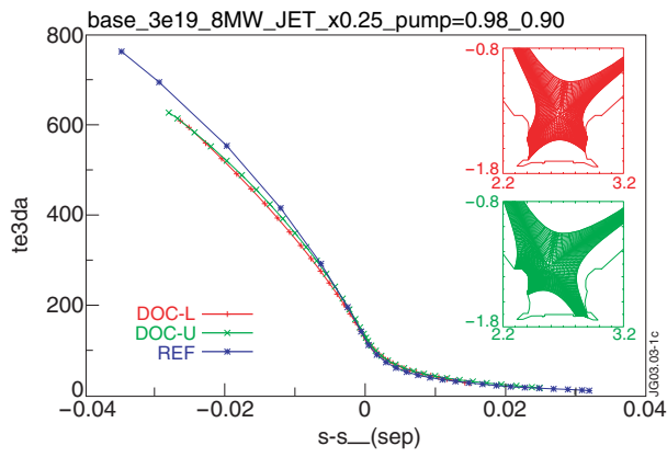
Figure 1. Upstream electron temperature profiles from a SOLPS5.0 B2-Eirene simulation. Inset are zooms of the divertor region of the DOC-L and DOC-U grids. (The reference grid is shown as an inset in figure 2.)
