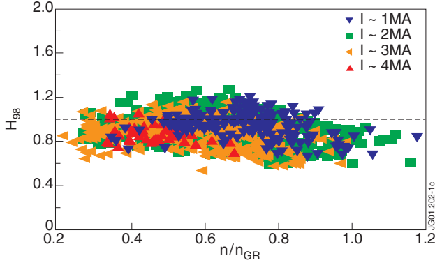
Figure 1: H_{98} ( \equiv \tau_{IH} / \tau_{E98} ) versus n/n_{GR} , the data are grouped by current I in MA 0.5 < I < 1.5 , 1.5 < I < 2.5 , 2.5 < I < 3.5 and I > 3.5 .
