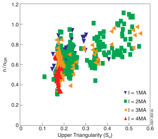
Figure 4: n/n_{GR} versus the upper triangularity \delta_u , current grouping as in Fig. 1.
