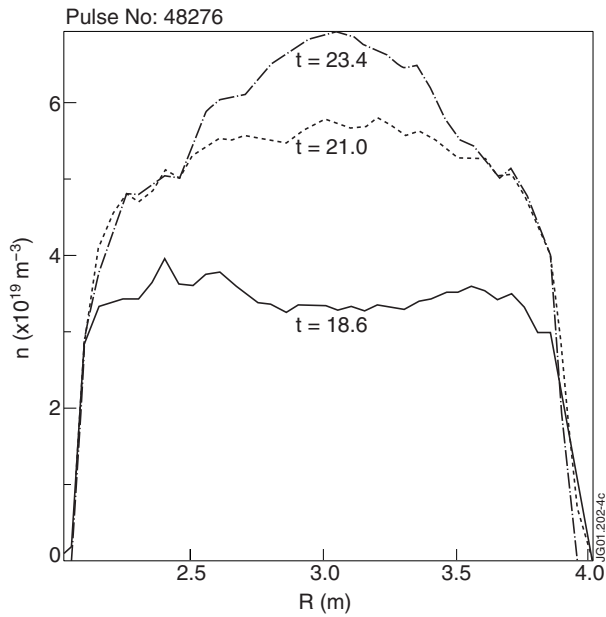
Figure 3: The electron density profile at three times.
