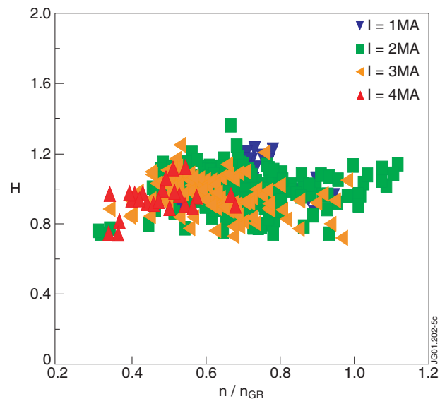
Figure 5: The fit for the H factor given by Eq. (4) versus n/n_{GR} .
