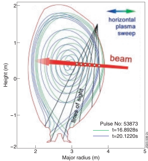
Figure 2: Flux surfaces (EFIT) for the extreme positions of the horizontal sweep.
