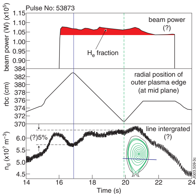
Figure 3: Time trace of injected beam power, plasma position and line integrated density during a sweep pulse.
