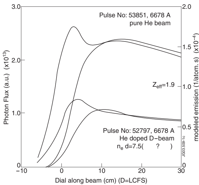
Figure 1: Comparison of given singlet beam emission profile for a doped D/H_e and a pure H_e beam.
