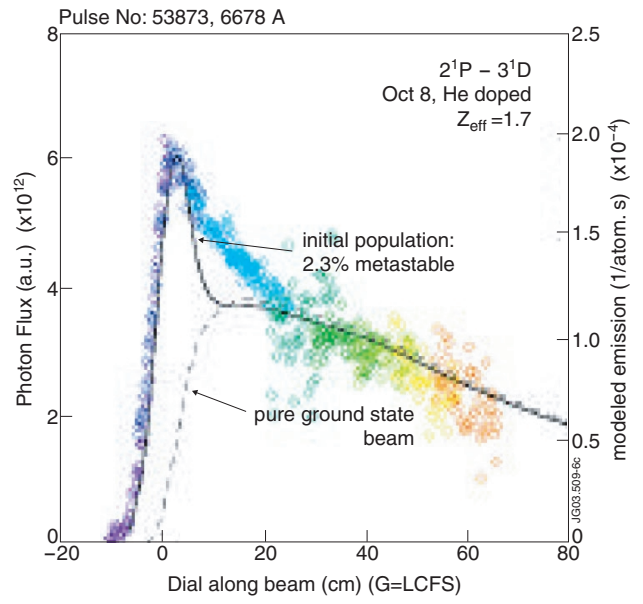
Figure 6: H_e I beam emission profile of the 2^1P-3^1D singlet line ( H_e doped beam 130keV).
