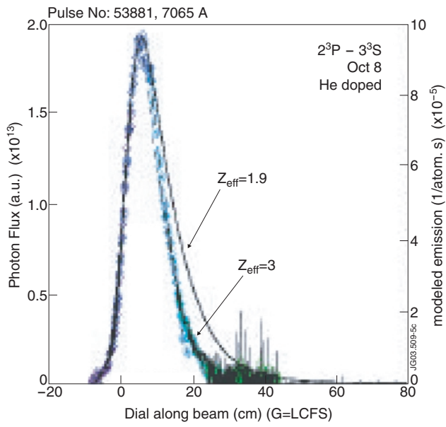
Figure 5: H_e I beam emission profile of the 2^3P-3^3S triplet line ( H_e doped beam 130keV).
