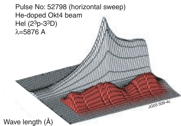
Figure 4: Beam emission profile showing the Doppler-shifted emission (right, red) and the unshifted emission (left) for a 6s doped 74kV beam.
