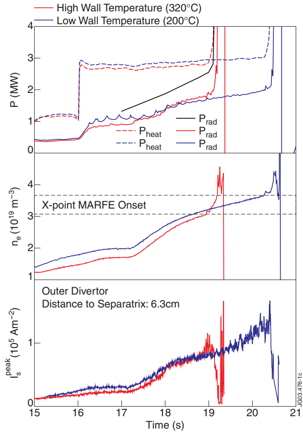
Figure 1: Comparison of two L-mode Pulse No's: (52684, 53077).
