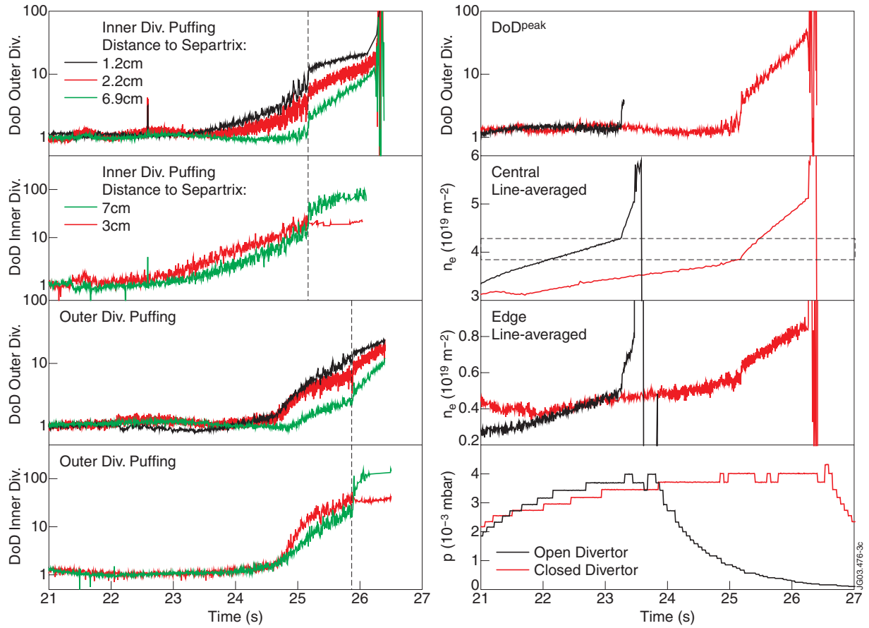
Figure 3: Left: Degree Of Detachment for inner divertor (53080) and outer divertor (53081) puffing in Closed divertor configuration; Right: Comparison of density limit in Open (53082) and Closed (53080) divertor configuration; X-point MARFE onset is indicated by dashed line.
