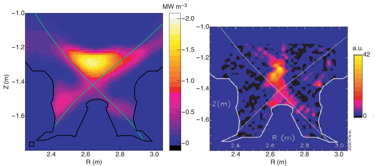
Figure 4: MARFE: comparison of bolometric tomographic reconstruction (left) with tomographic reconstruction of CIII line emission (right); 53080 at 26s.
