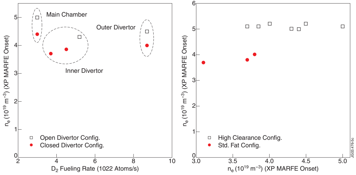
Figure 5: Summary of X-point MARFE onset and Wall MARFE onset for L-mode density limit discharges.
