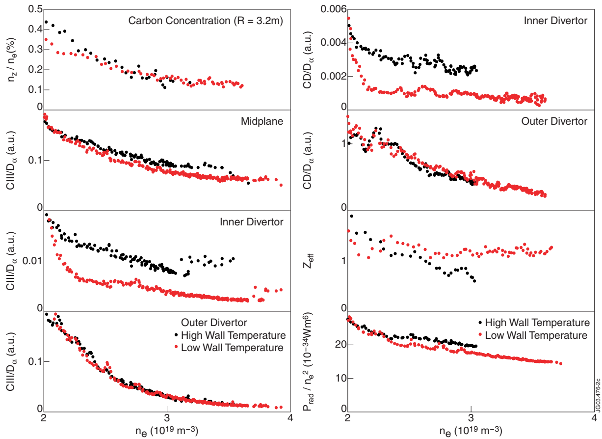
Figure 2: Carbon release: Normalized photon fluxes CIII/D_\alpha and CD/D_\alpha , Z_{eff} carbon concentration from CXRS.
