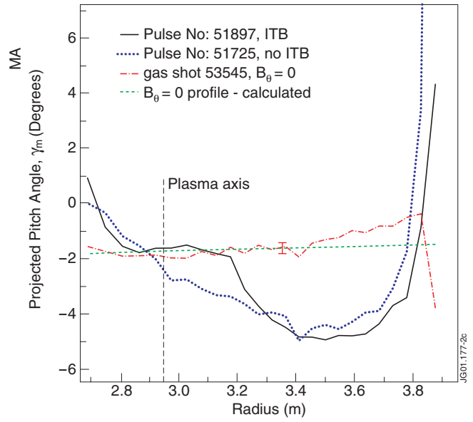
Figure 2: Profiles of projected pitch angle, \gamma_m , obtained with the MSE diagnostic, showing the appearance of a flat region near the plasma axis. This is interpreted as zero toroidal current.
