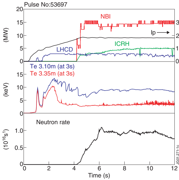
Figure 1: Time history of plasma parameters for a typical reversed shear experiment. Note the ‘sawtooth-like’ collapses on the Te signals between 2 and 4 seconds.
