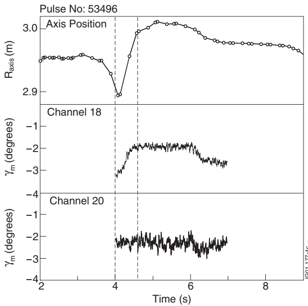
Figure 3: The plasma is moved radially by 10cm between 4.0–4.6s. Channel 20 remains in the region of zero poloidal field during the entire sweep and records no change.
