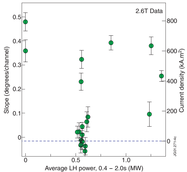
Figure 4: Slope of the flat region in the m profiles for a number of discharges. There is evidence that the axis current, although reduced to zero, is never driven below zero.
